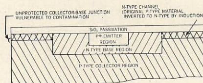
Cross Section of Planar Transistor
