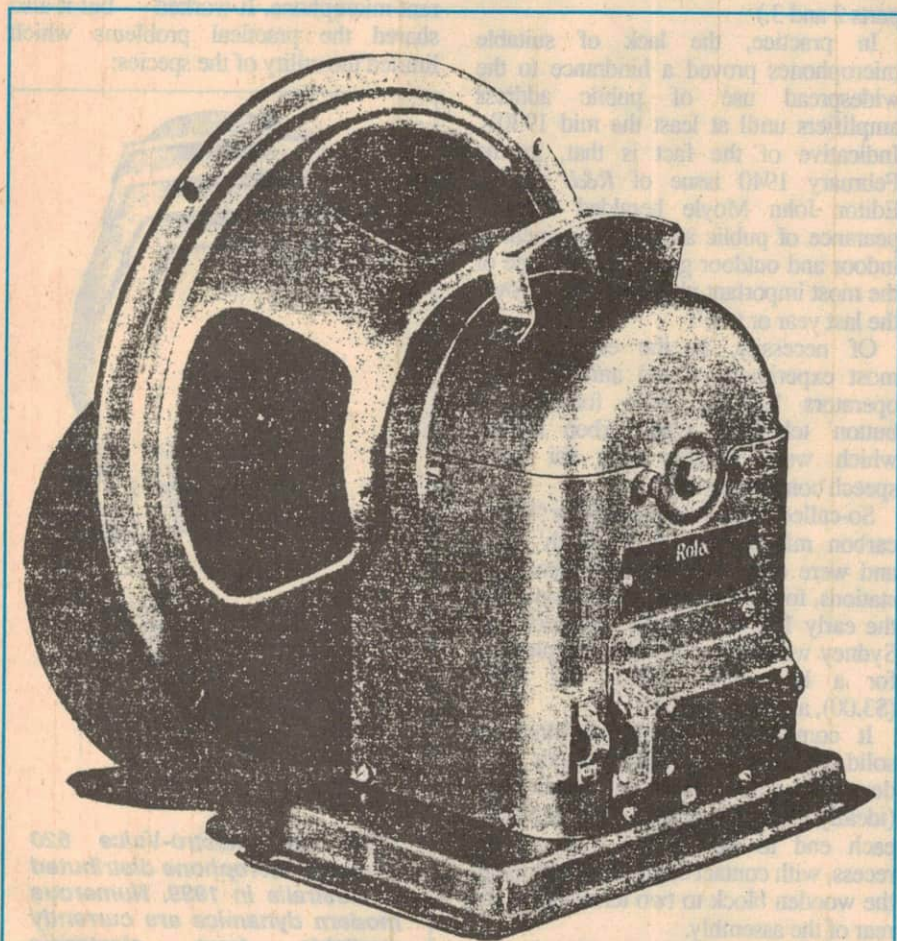
Fig.4: The Rola G-12 electrodynamic loudspeaker, as advertised in R&H for March, 1942 'For Public Address'. The retail price was quoted as £9 ($18) — which represented a much larger outlay than it sounds today!
