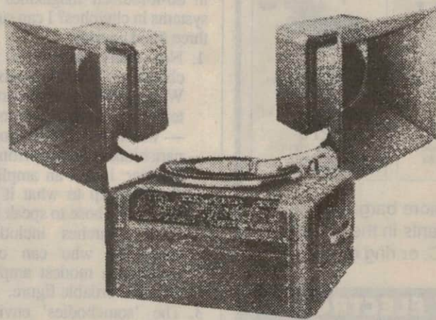
Fig.6: From R&H for September 1939, one of a series of Webster-Chicago PA amplifiers distributed in Australia by International Radio Pty Ltd. Power outputs ranged from 8 - 60W. The loudspeakers used 12-inch (30cm) drivers in small wooden cabinets with frontal flares.
