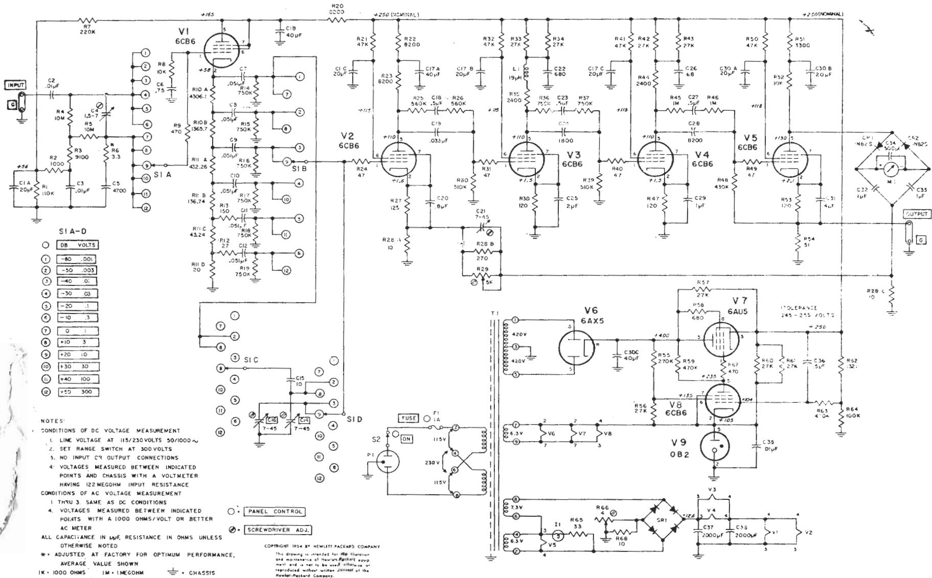
hp MODEL 400D VACUUM TUBE VOLTMETER SERIAL 5131 & ABOVE
