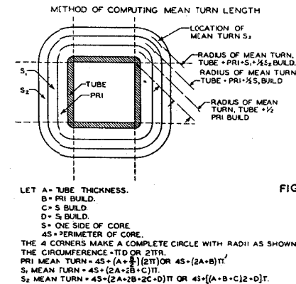
Fig. 5.18D. Method of computing mean length of turn (Ref. D20).
