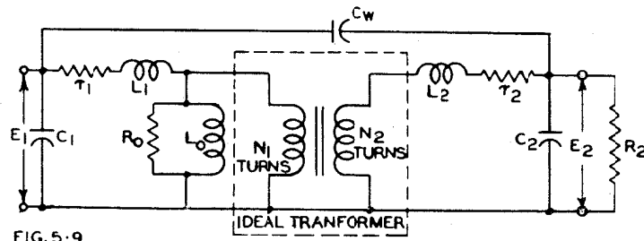
Fig. 5.9. Equivalent circuit of a practical transformer.
