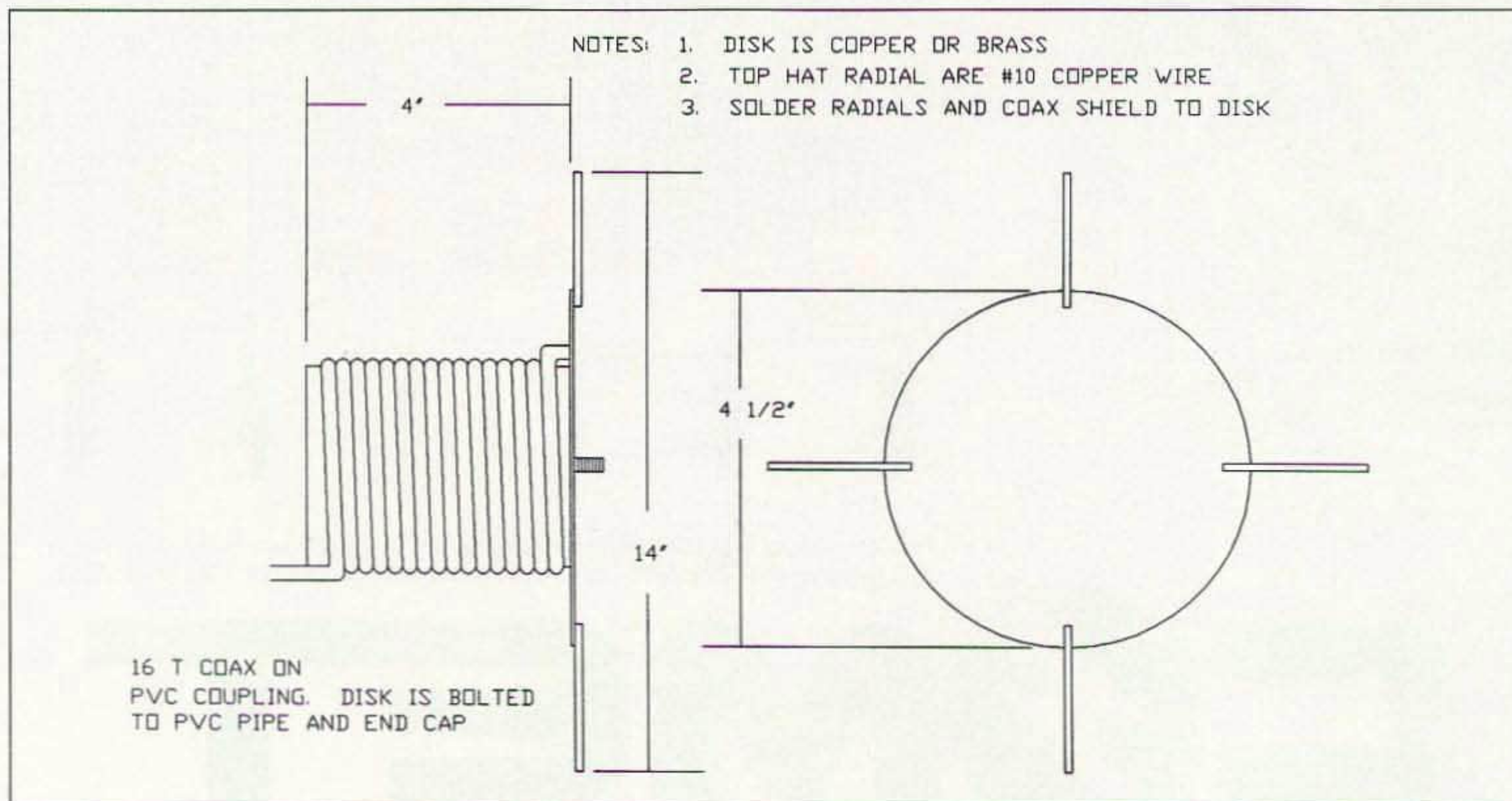
Figure 4. 20 meter resonator.
