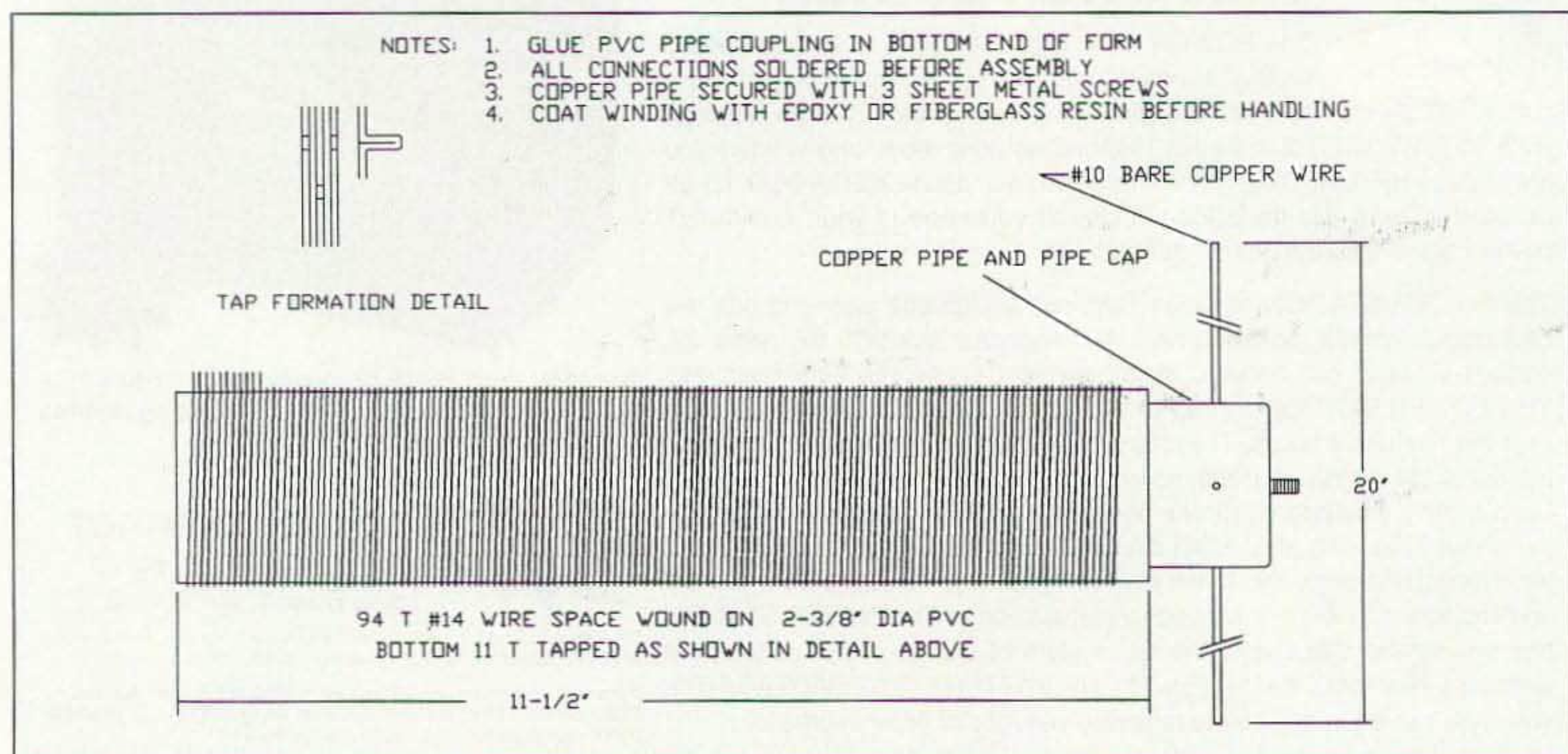
Figure 2. 75 meter resonator.
