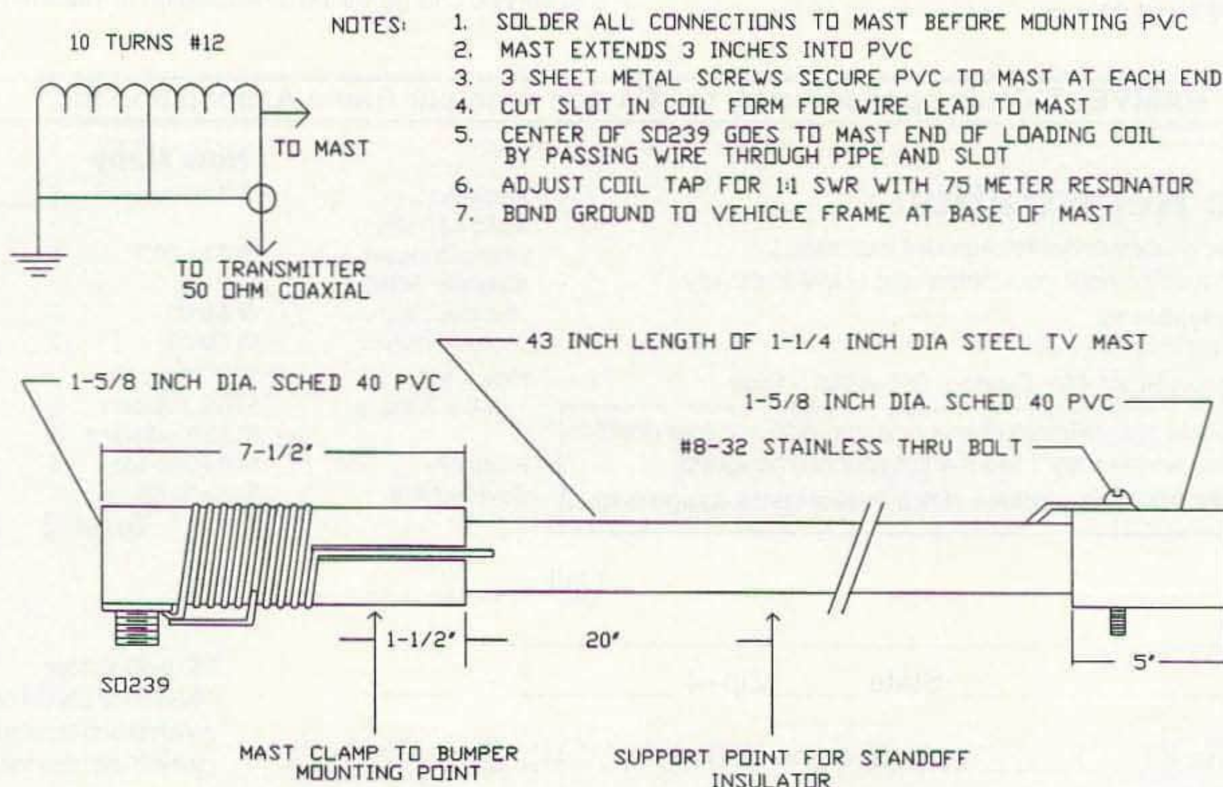
Figure 1. Mobile mast construction detail.
