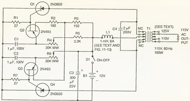
Fig. 29-1. DC-to-AC inverter.
