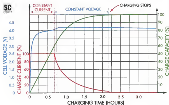
Fig.3: graphs showing the safe charging protocol recommended for single Li-ion cells and batteries with the cells connected in parallel.
