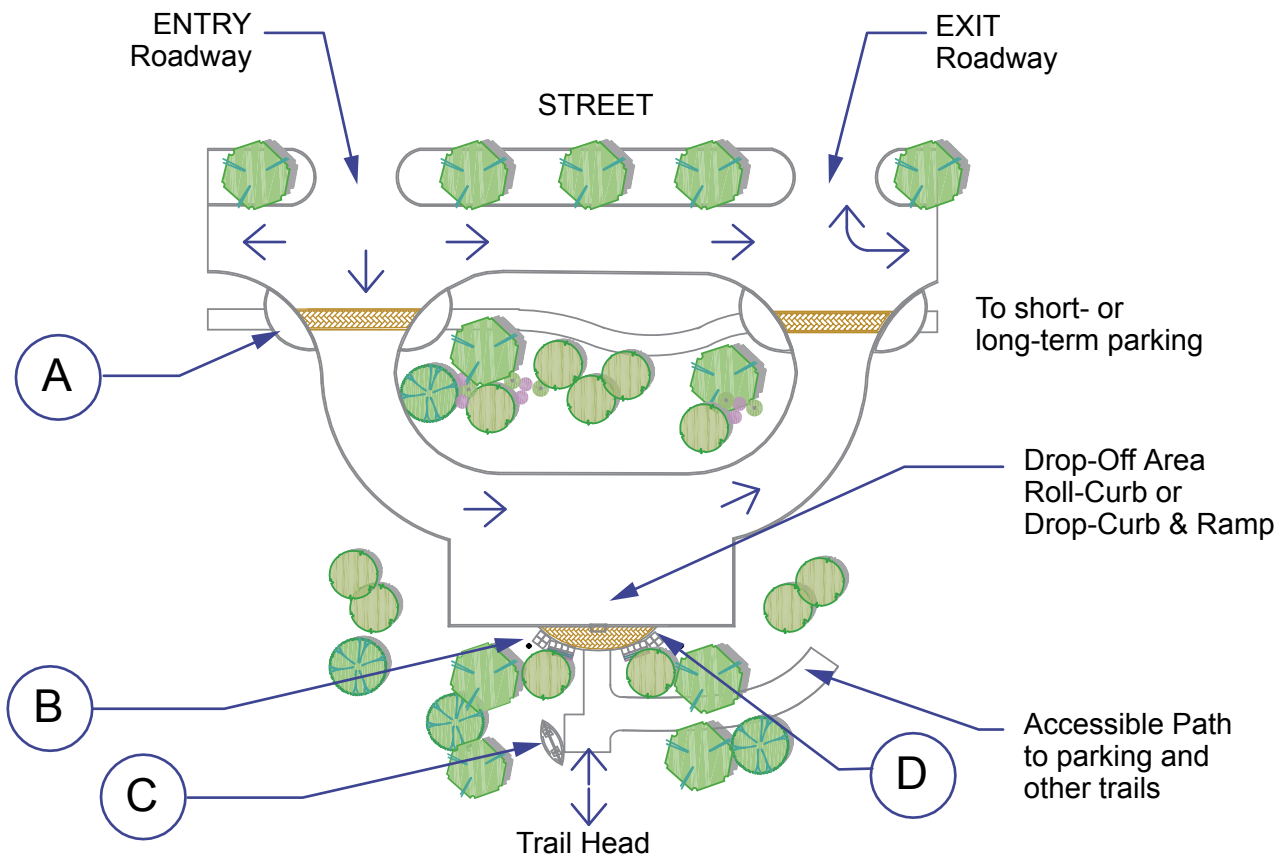
Figure 3.14 – Drop-Off & Pick-Up Areas
