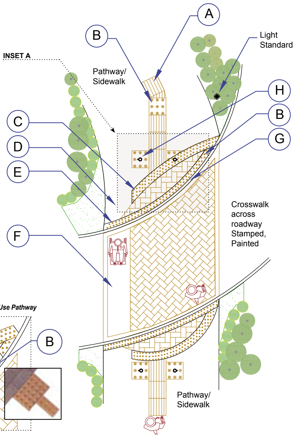
Figure 3.9 – Universal Multi-Use Pathway Crosswalk
