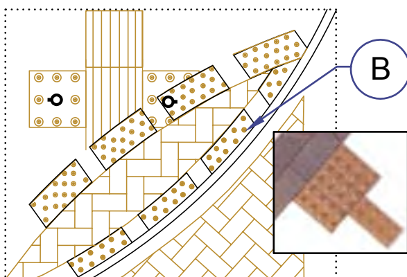
Figure 3.9.A – INSET Universal Multi-Use Pathway
