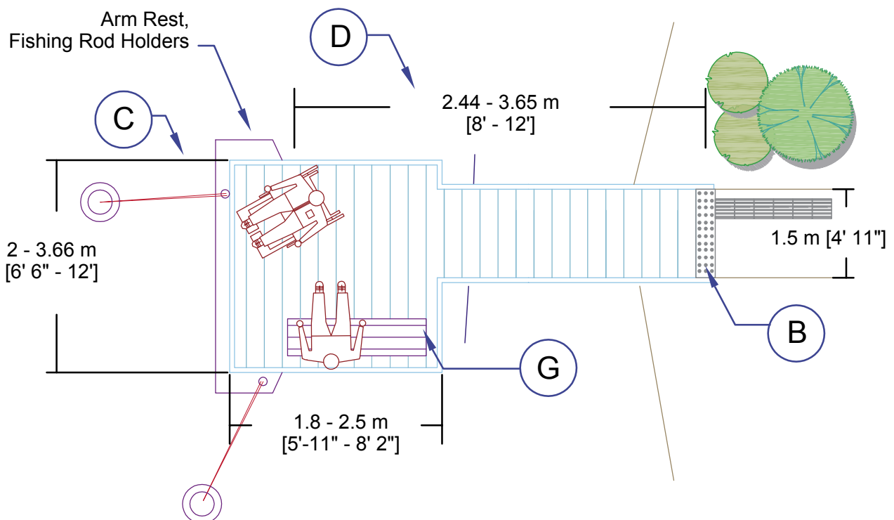
Figure 3.25 – Fishing Dock Plan View
