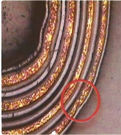
The thicker a circuit is, the less it can flex without damage. Here a hairline crack has formed in an outer trace from a bend radius that was too tight.
