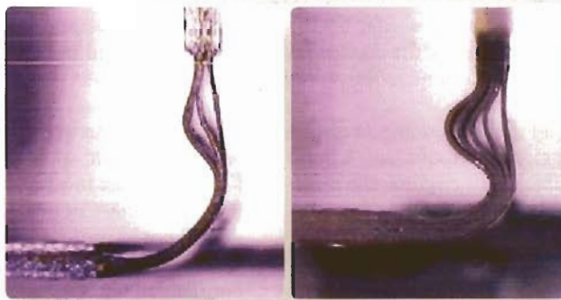
Potentially damaging forces can sometimes be reduced by unbonding layers in the bend area, as shown on the left. However, if the unbonded area is too short, buckling can lead to unacceptably tight bend radii as shown on the right.
