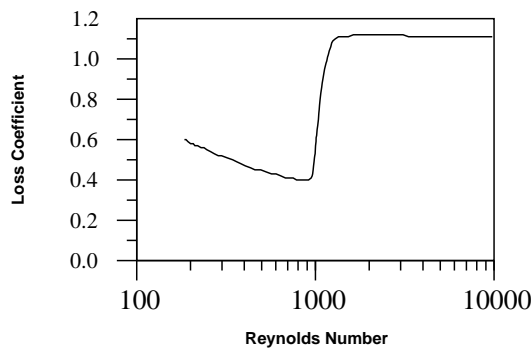
Figure 4.3: The results for the flow in a pipe with orifice
