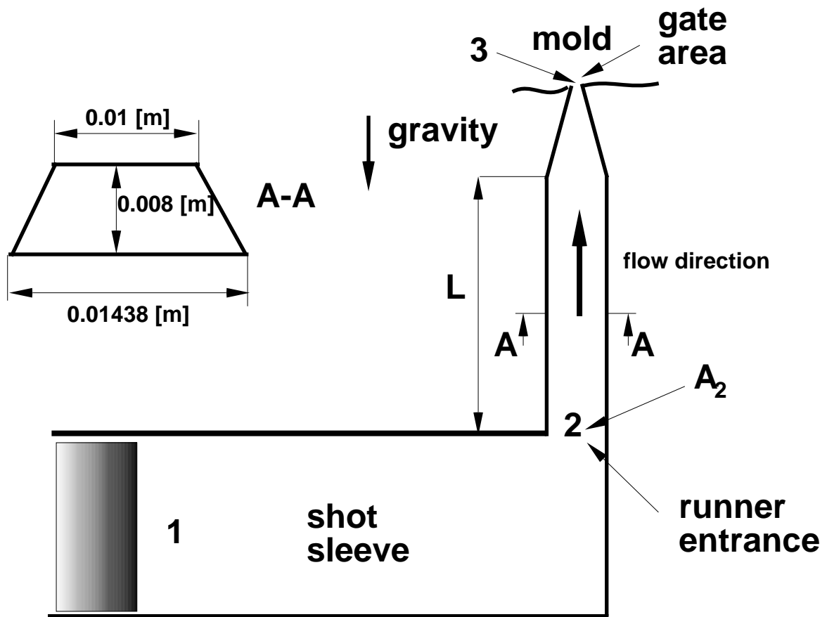
Figure 7.10: Design and dimensions of the runner for the example 7.4.2. The length, L , represents different runner design qualities. The gate design is made of straight lines to the gate area, creating a symmetrical gate.
