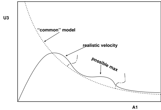
Figure 7.20: The gate velocity, U_3 as a function of the plunger area, A_1
