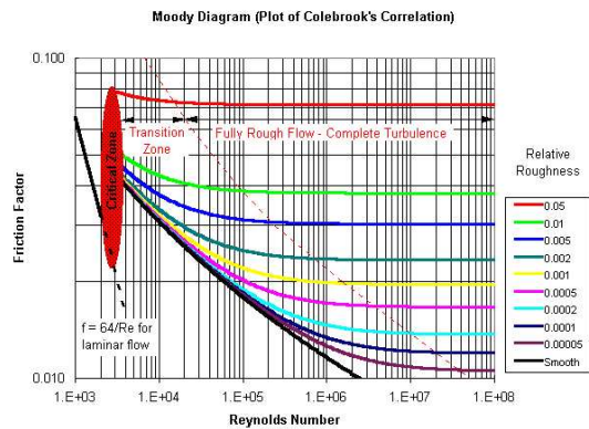
Figure 4.5: Moody's diagram
