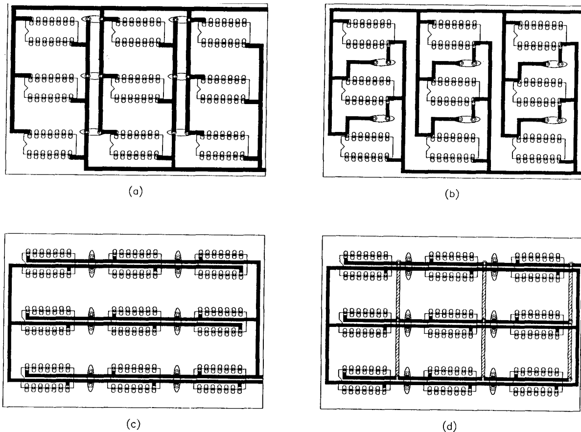
Figure 2 Power and ground bussing on two-sided boards
