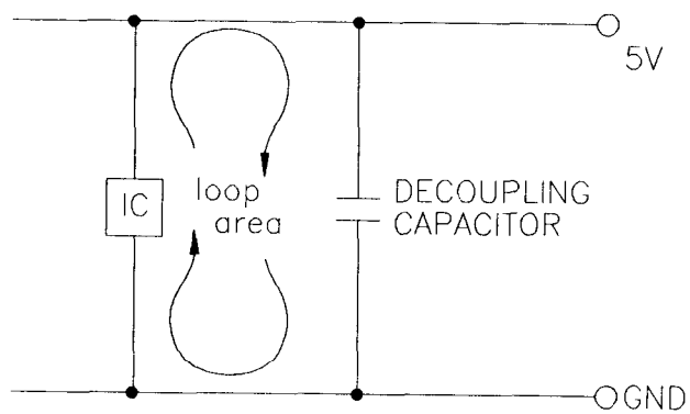
Figure 3 Bypass capacitor should be close to the ICS they serve to reduce the loop area and inductance.
