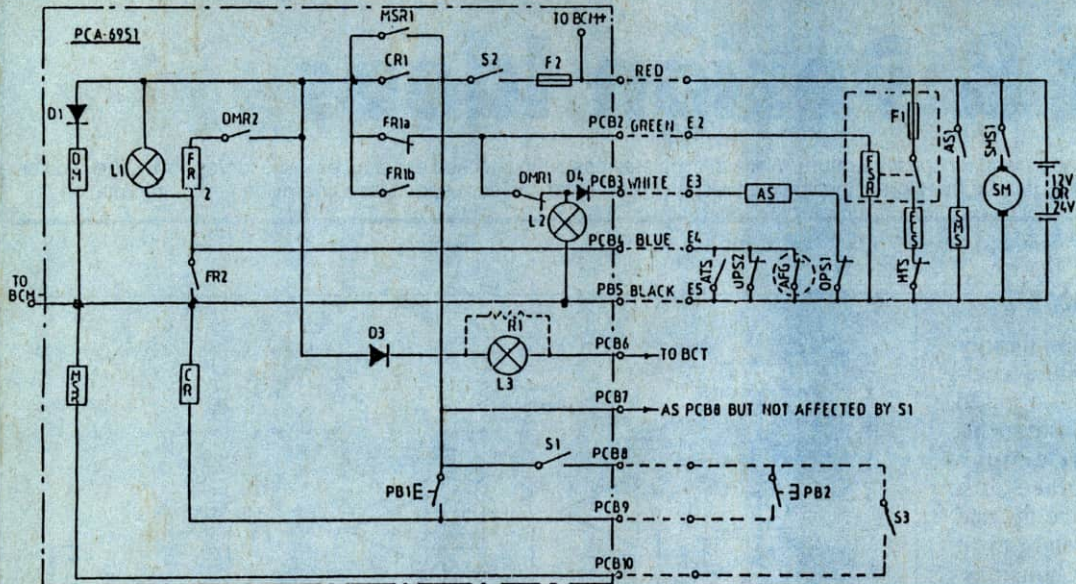
The circuit diagram for the control system of the 7.5kVA Lister diesel generator set which Peter Laughton had to repair.
