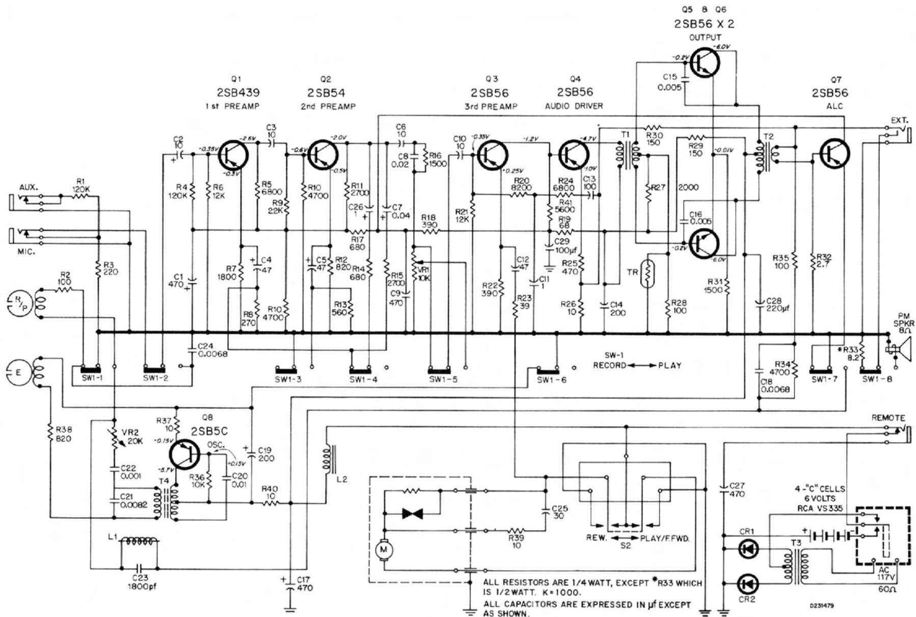
Fig. 5-56. RCA Model YZB525 tape recorder. (Courtesy RCA)
