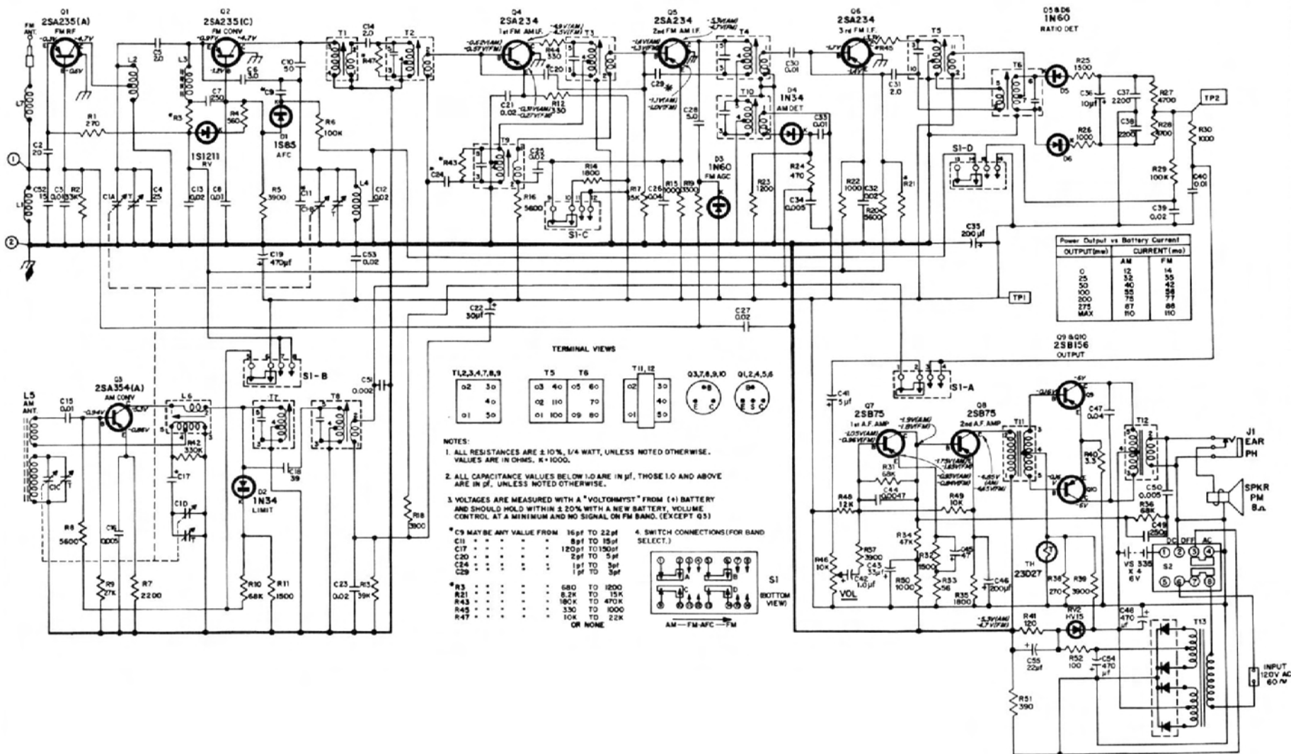
Fig. 5-24. RCA Model RZM170 AM-FM radio. (Courtesy RCA)
