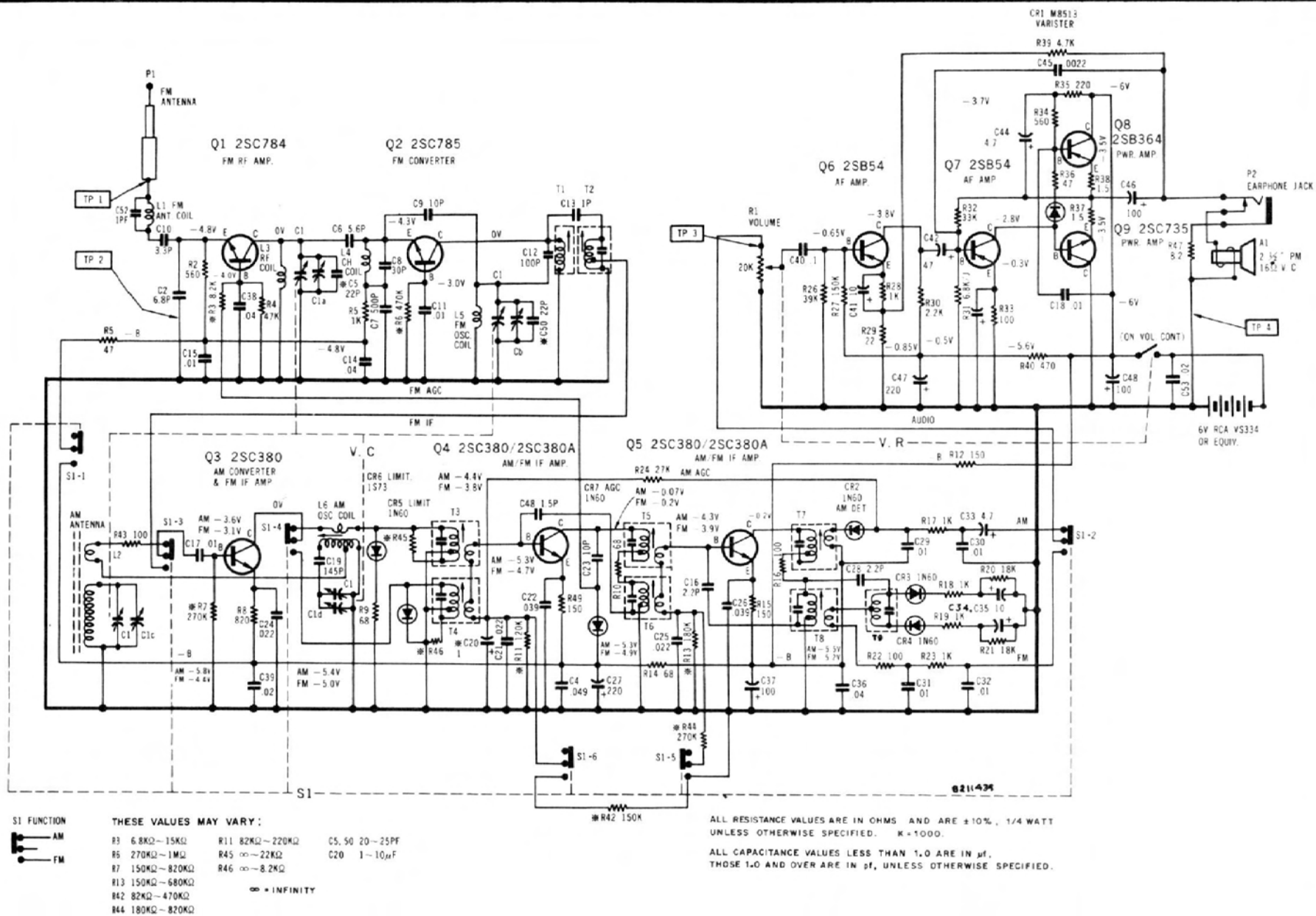
Fig. 5-22. RCA Model RZM160 AM-FM radio (Courtesy RCA)
