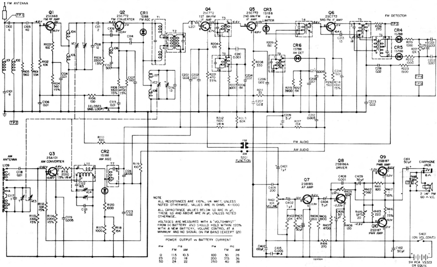
Fig. 5-20. RCA Model RZM145, 150 AM-FM portable radio. (Courtesy RCA)
