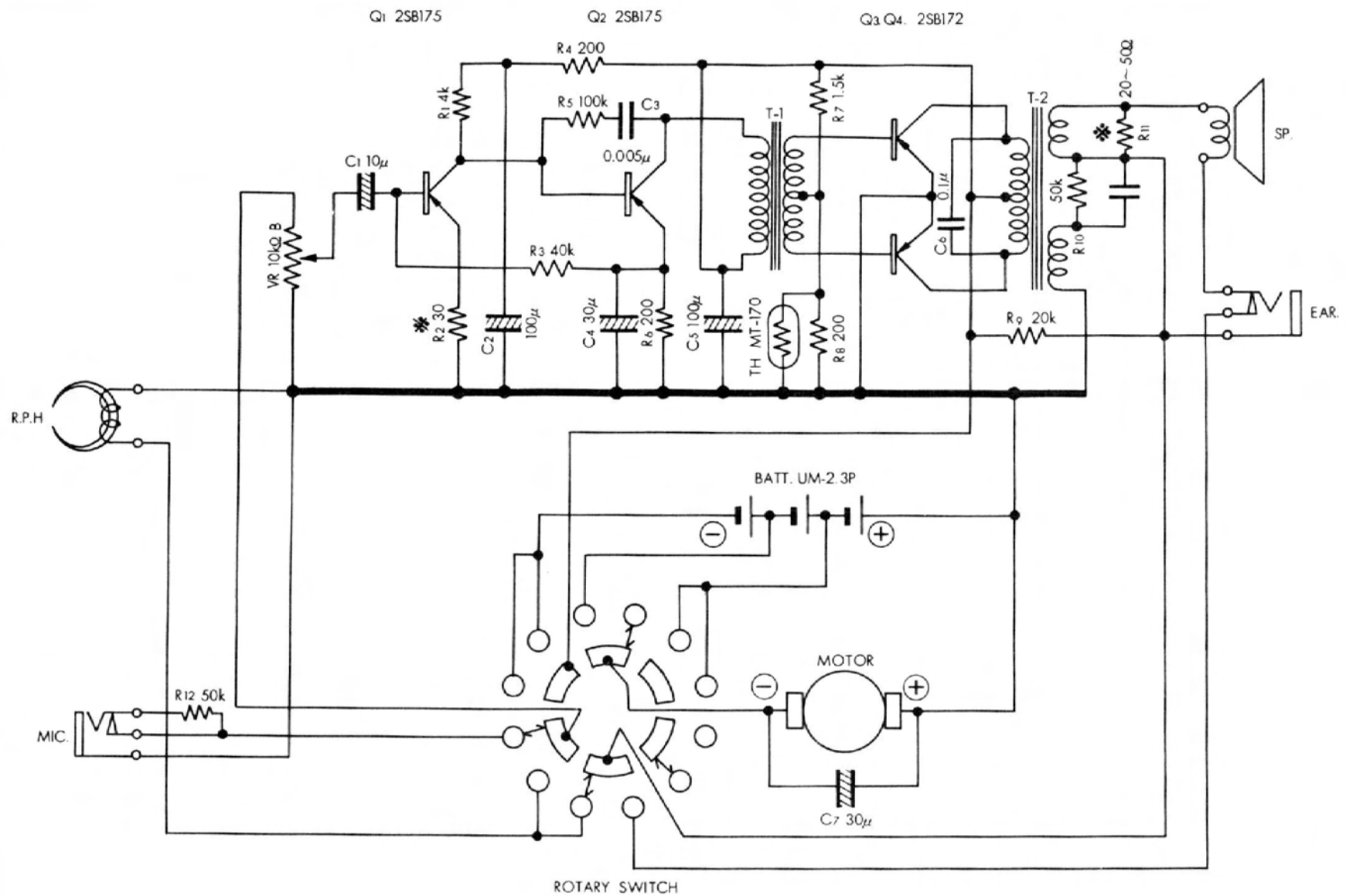
Fig. 5-46. Penncrest Model 6315 3-inch reel-type recorder. (Courtesy J. C. Penney Co.)
