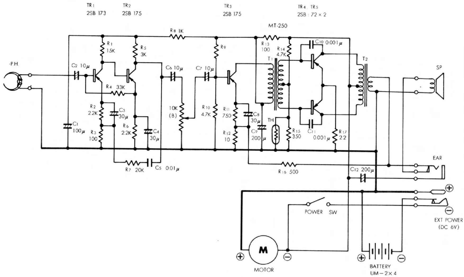
Fig. 5-44. Penncrest Model 3110 portable tape player. (Courtesy J. C. Penney Co.)
