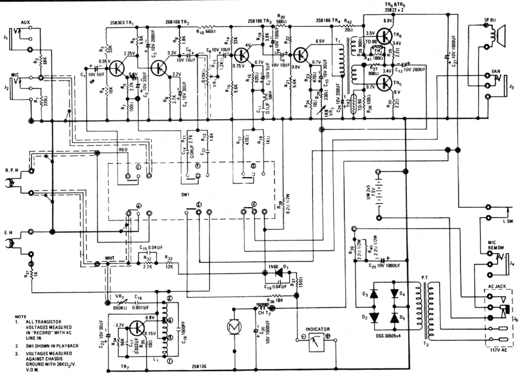
Fig. 2-11. Schematic diagram of the Mercury Model TR-5000 solid-state cassette tape recorder. (Courtesy Mercury Record Productions, Inc.)
