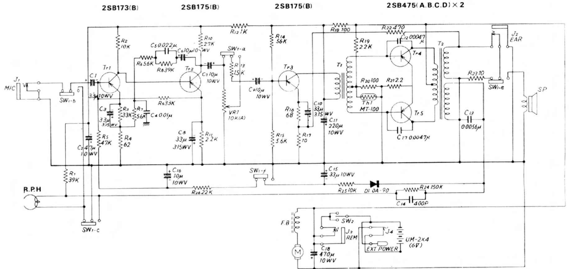
Fig. 5-41. Mercury Model 20-1002 tape recorder. (Courtesy Mercury Record Productions, Inc.)
