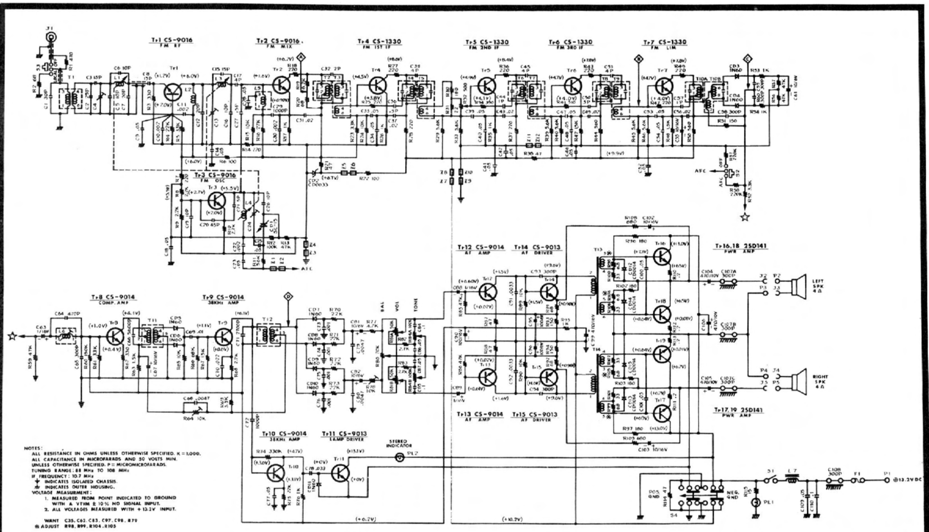
Fig. 5-34. Medallion Model 65-230 FM stereo multiplex auto radio. (Courtesy Midland International Corp.)
