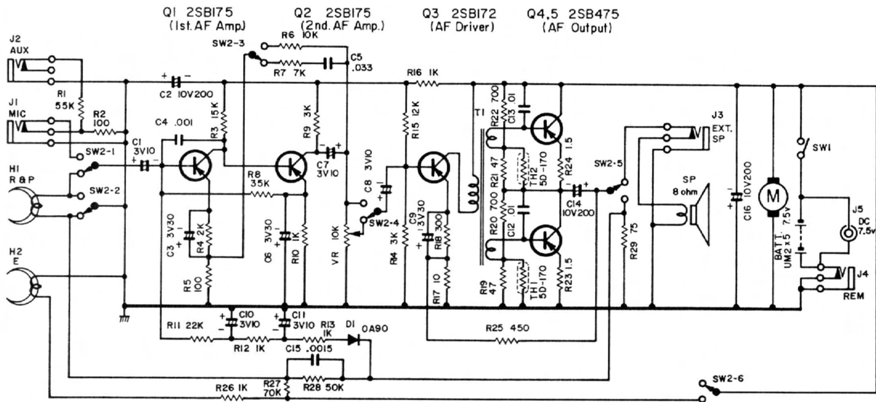
Fig. 5-40. Lloyd's Model 9V95-114A portable cassette tape recorder. (Courtesy Lloyd's Electronics, Inc.)
