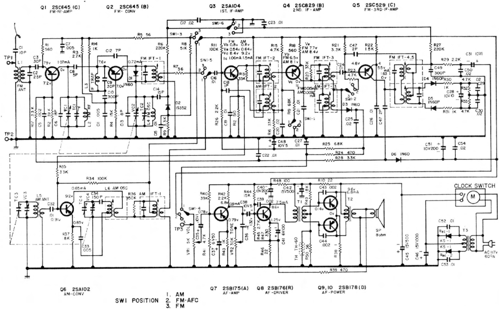
Fig. 5-15. Lloyd's Model 9J41-100A AM-FM radio. (Courtesy Lloyd's Electronics, Inc.)
