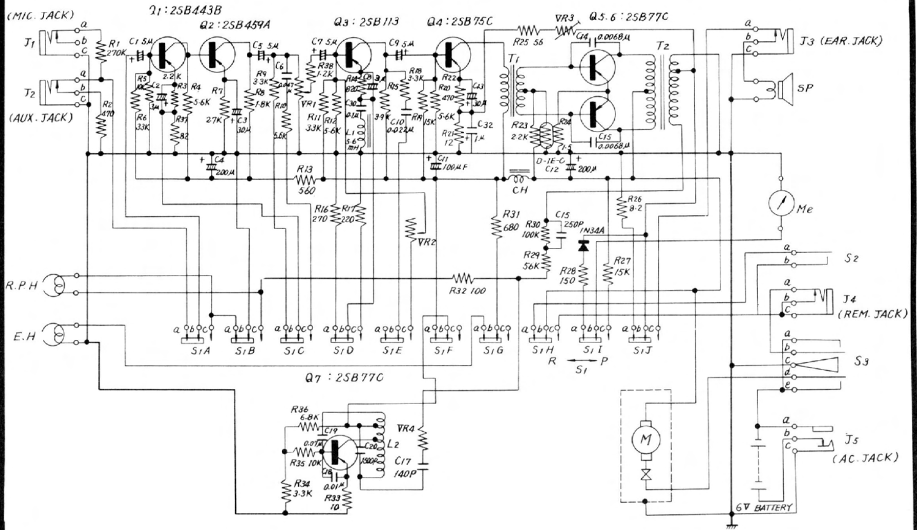
Fig. 5-38. Crown Model CTR-9000A tape recorder. (Courtesy Crown Radio Corp.)
