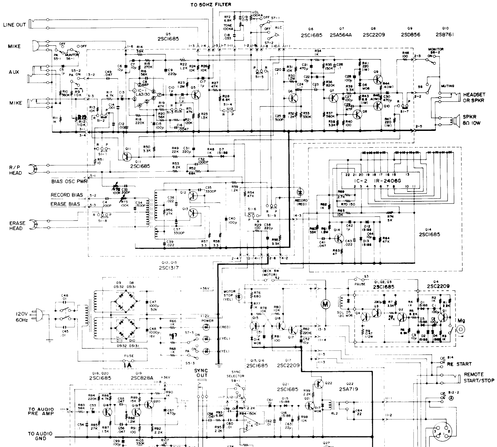
MODEL 162S-2 SCHEMATIC
