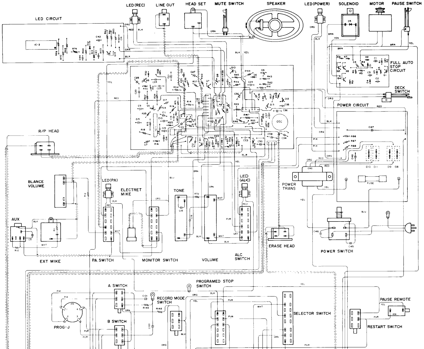
MODEL 162S-2 COMPONENT LAYOUT DIAGRAM
