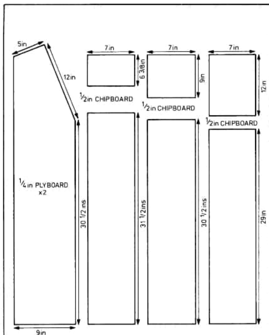
Figure 6: The cutting diagram for a single QWL loudspeaker (the baffle plate is also needed and is shown in Figure 7).
