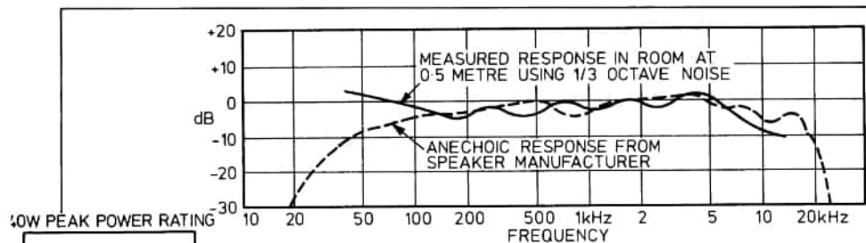
Figure 8: Frequency response of complete loudspeaker systems.
