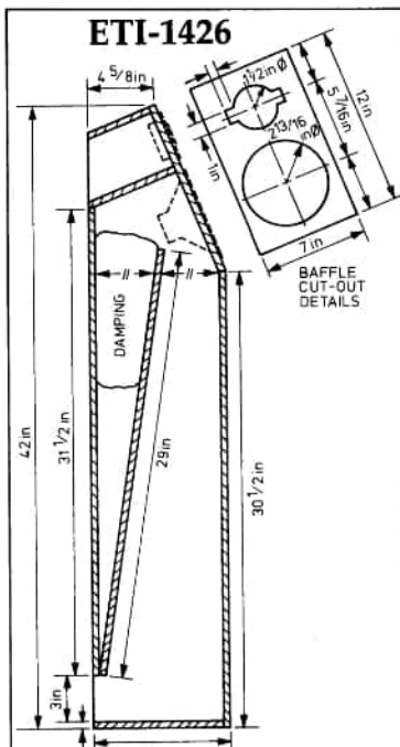
Figure 7: Enclosure dimensions and construction.
