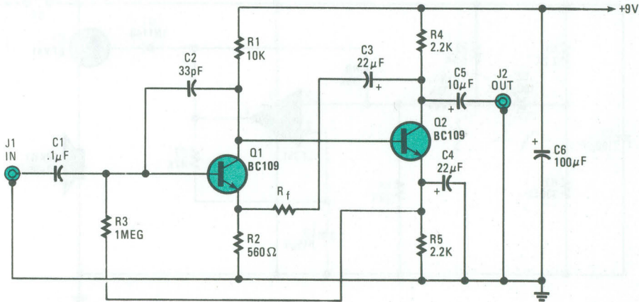
GENERAL-PURPOSE PREAMPLIFIER
