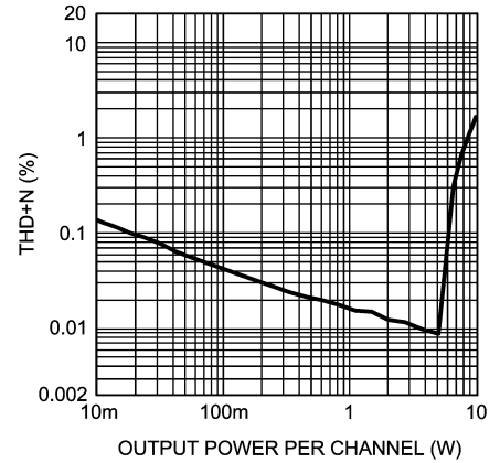
THD+N vs Output Power Per Channel V_{DD} = 12V, f_{IN} = 20Hz, R_L = 8\Omega
