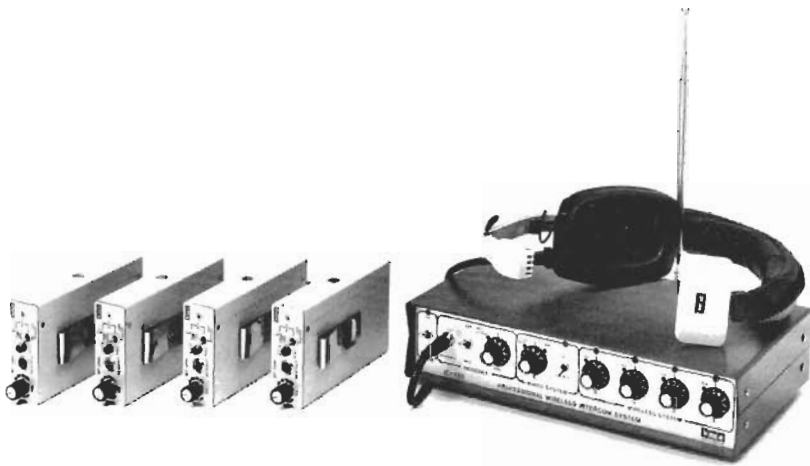
Wireless intercom provides full-duplex (simultaneous) conversation between five users, interfaces with popular wired intercoms for wider communications flexibility. This model has dynamic expansion for 85 dB dynamic range, especially useful in high-noise environments.
