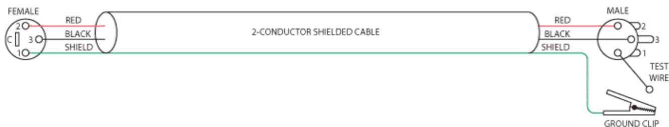
Figure 3. Test cable
