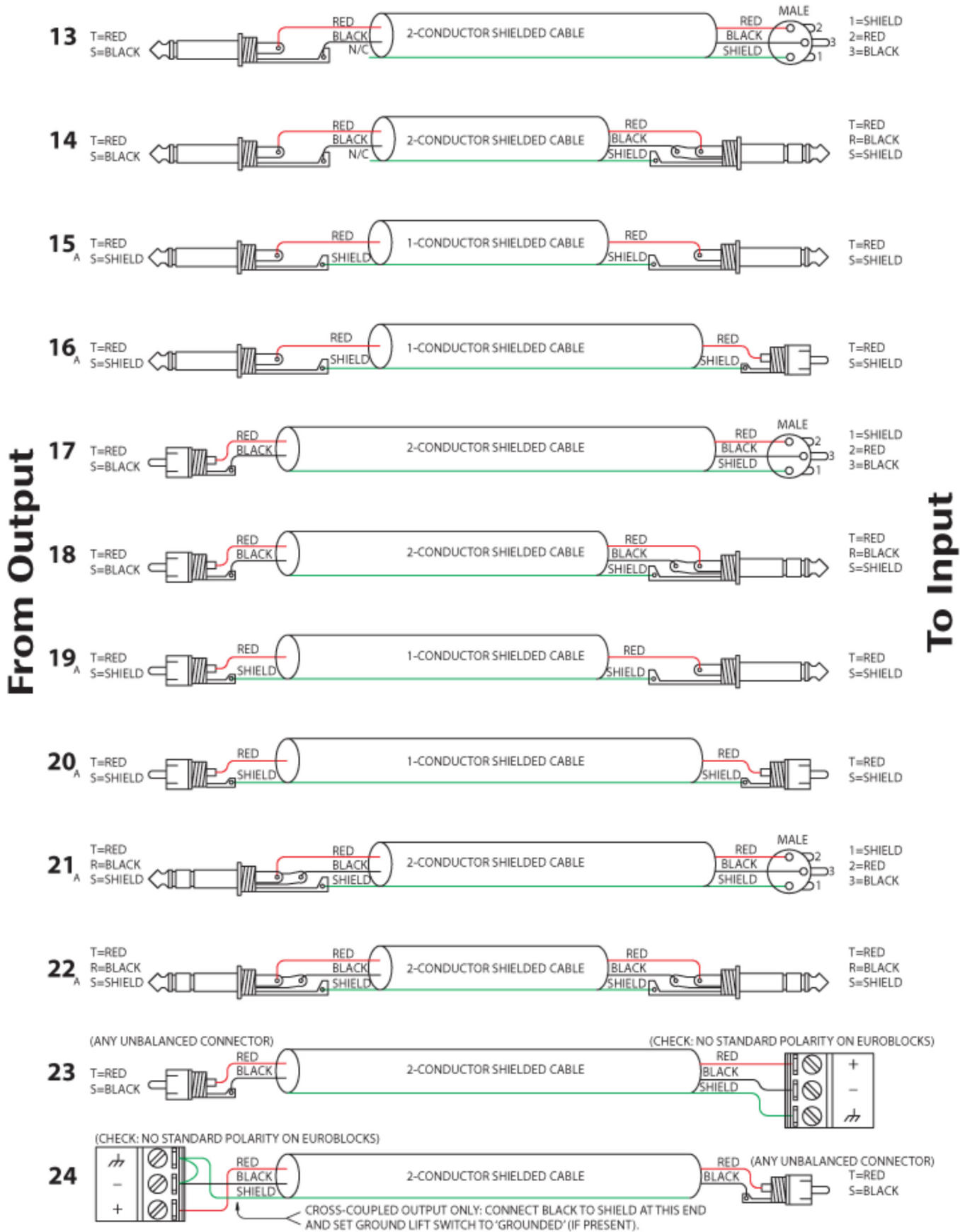
Figure 4. Interconnect chart for locating correct cable assemblies.
