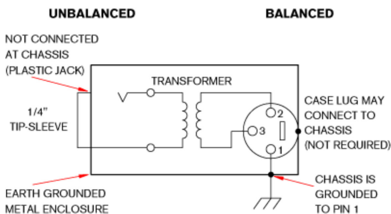
Figure 2. Transformer Isolation
